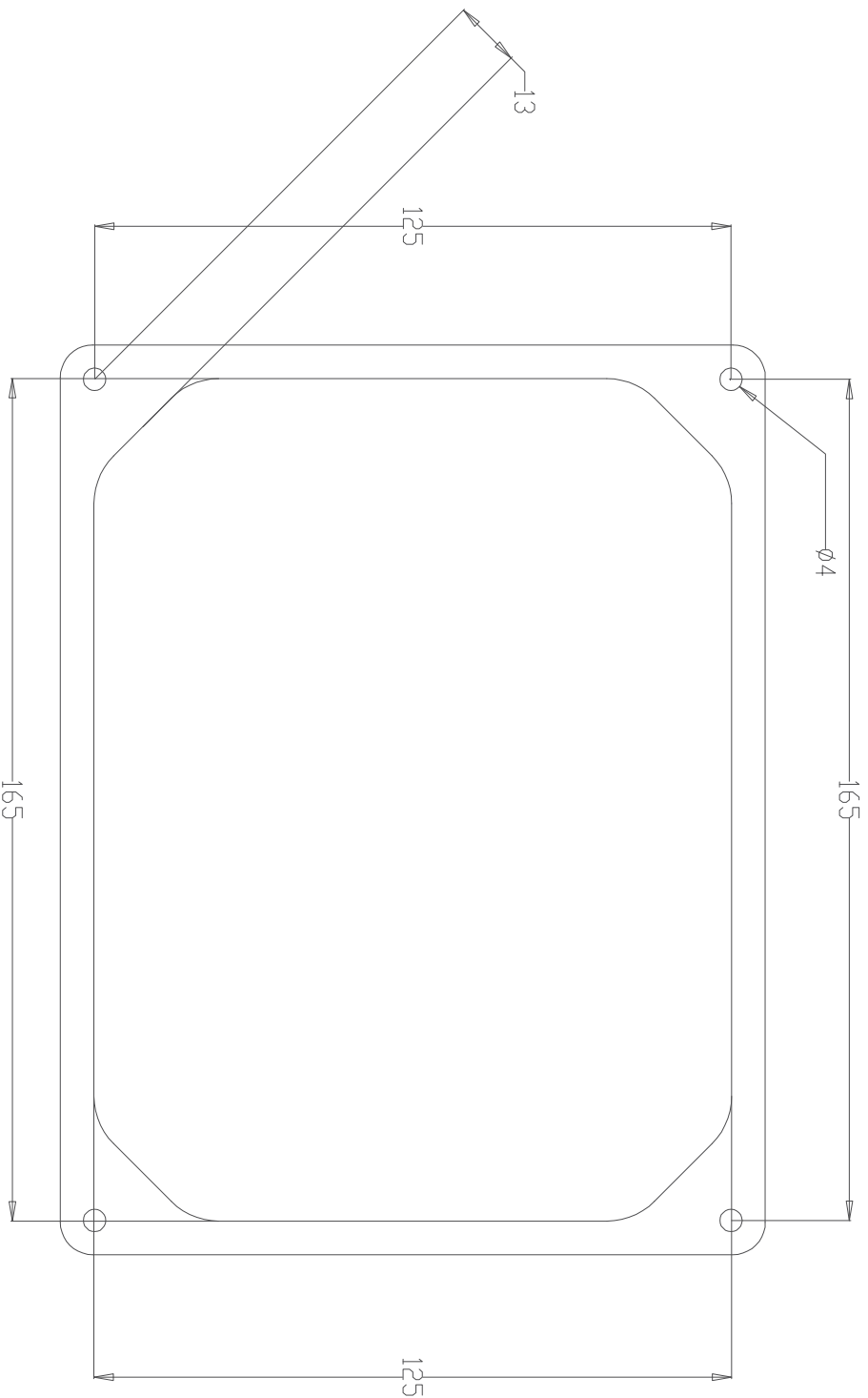
"B" PANEL CUT TEMPLATE
