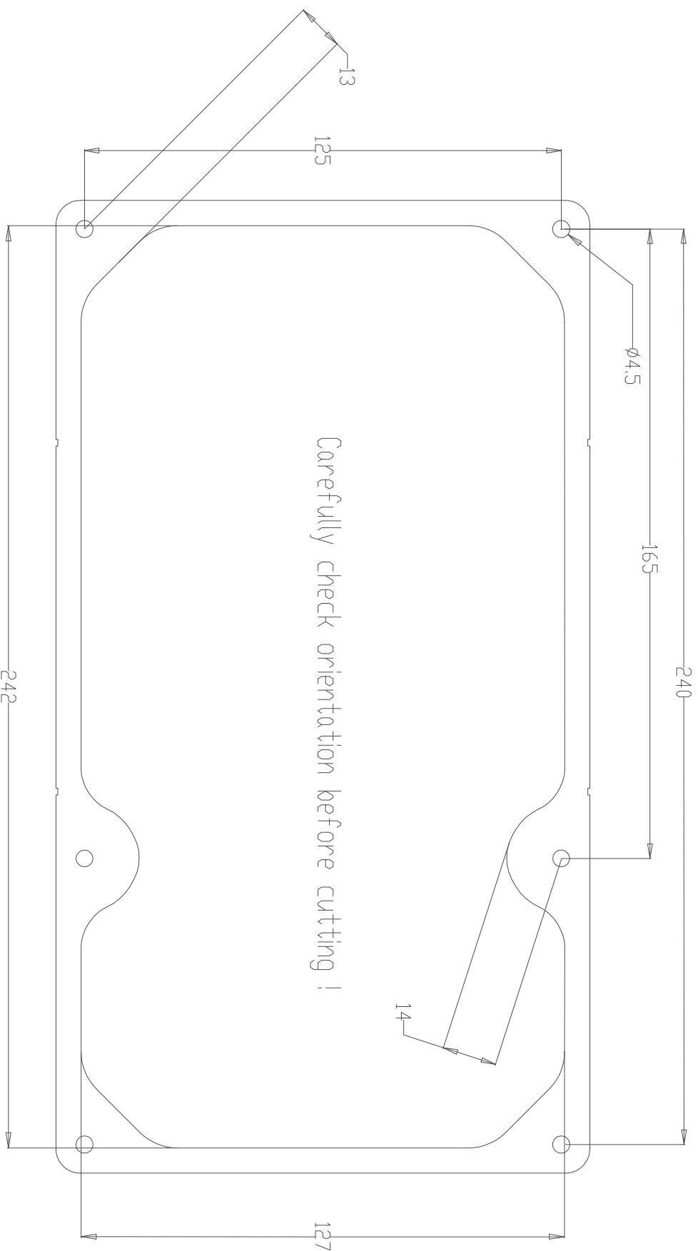
C PANEL CUTOUT TEMPLATE
